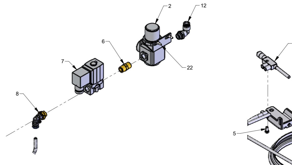
DETAIL B (1 : 4)
