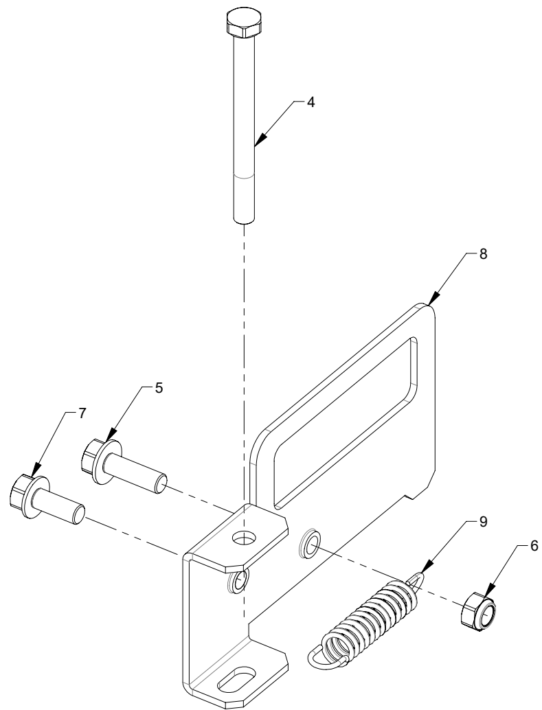
DETAIL A (1 : 2)
