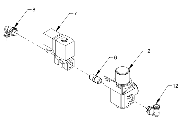
DETAIL A (1 : 4)
